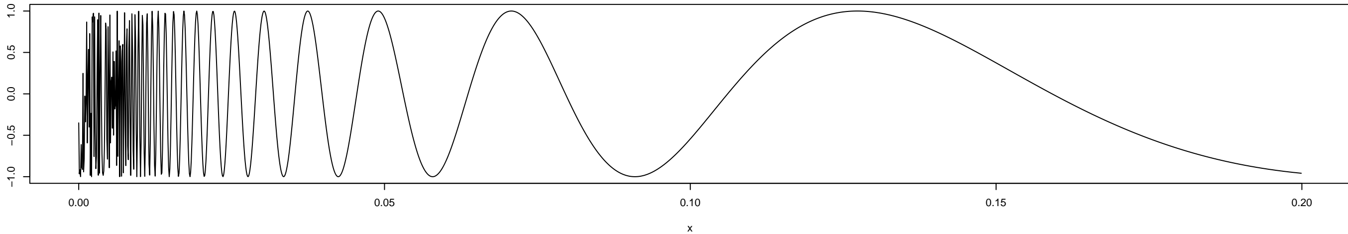
sin(1/x)
