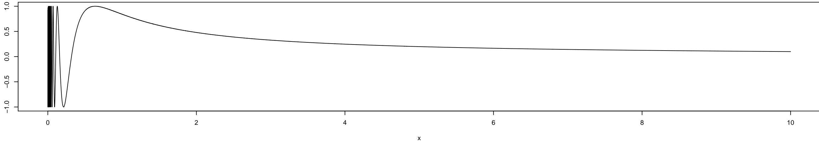
sin(1/x)
